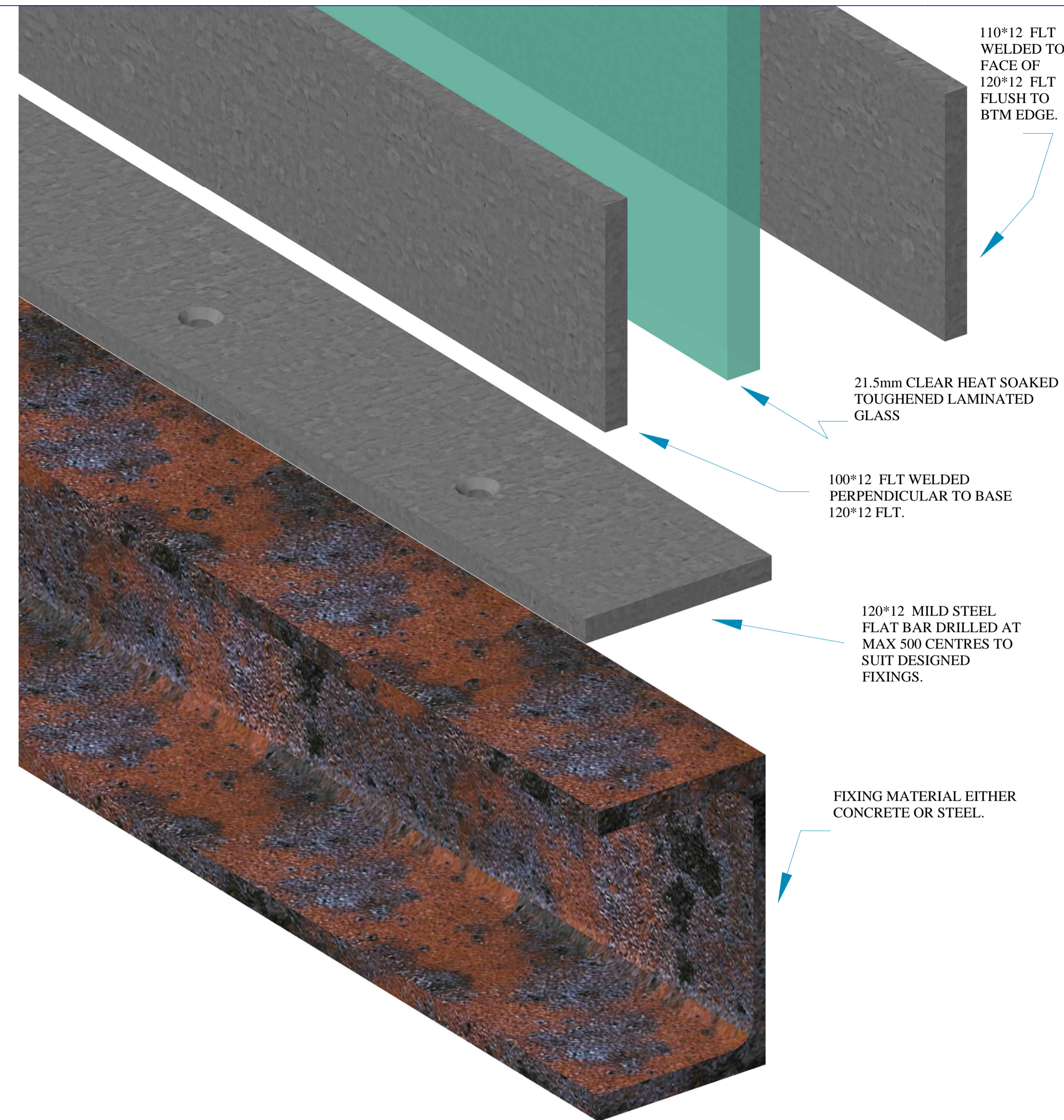
EXPLODED VIEW
