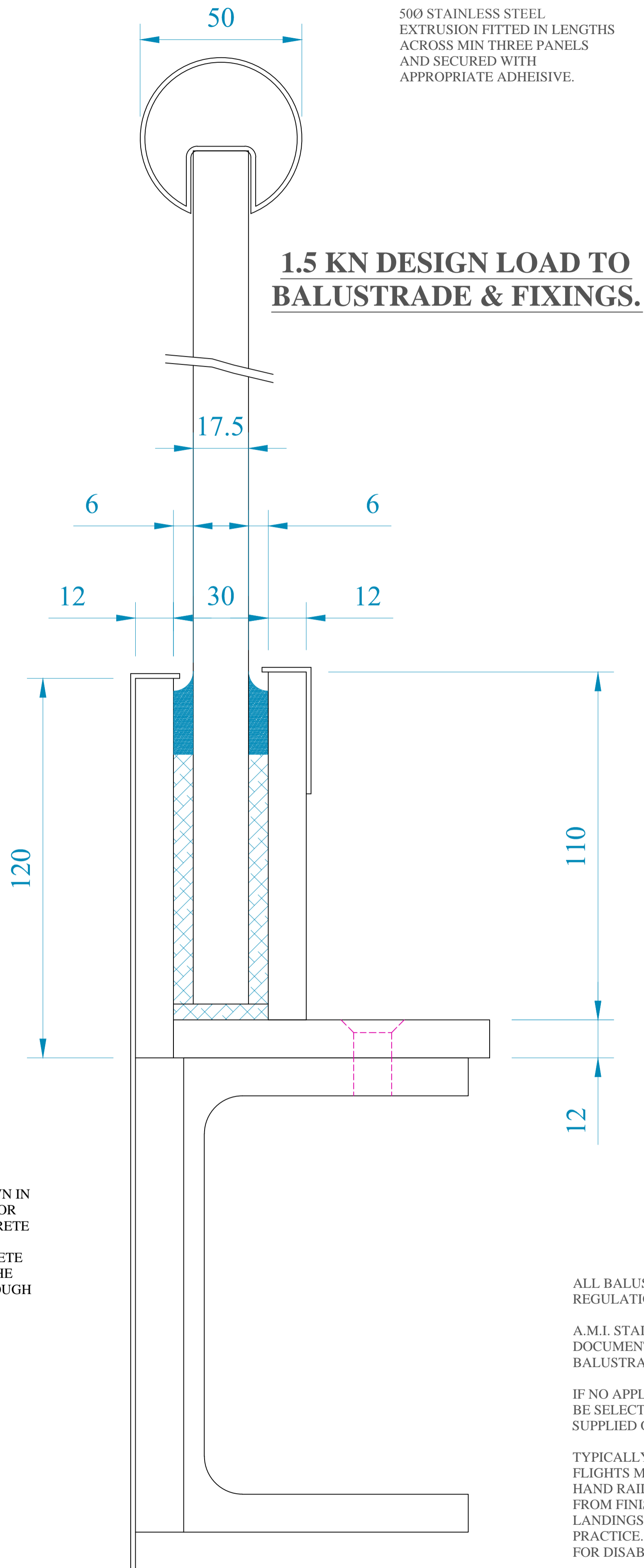
TYPICAL SECTION THROUGH
